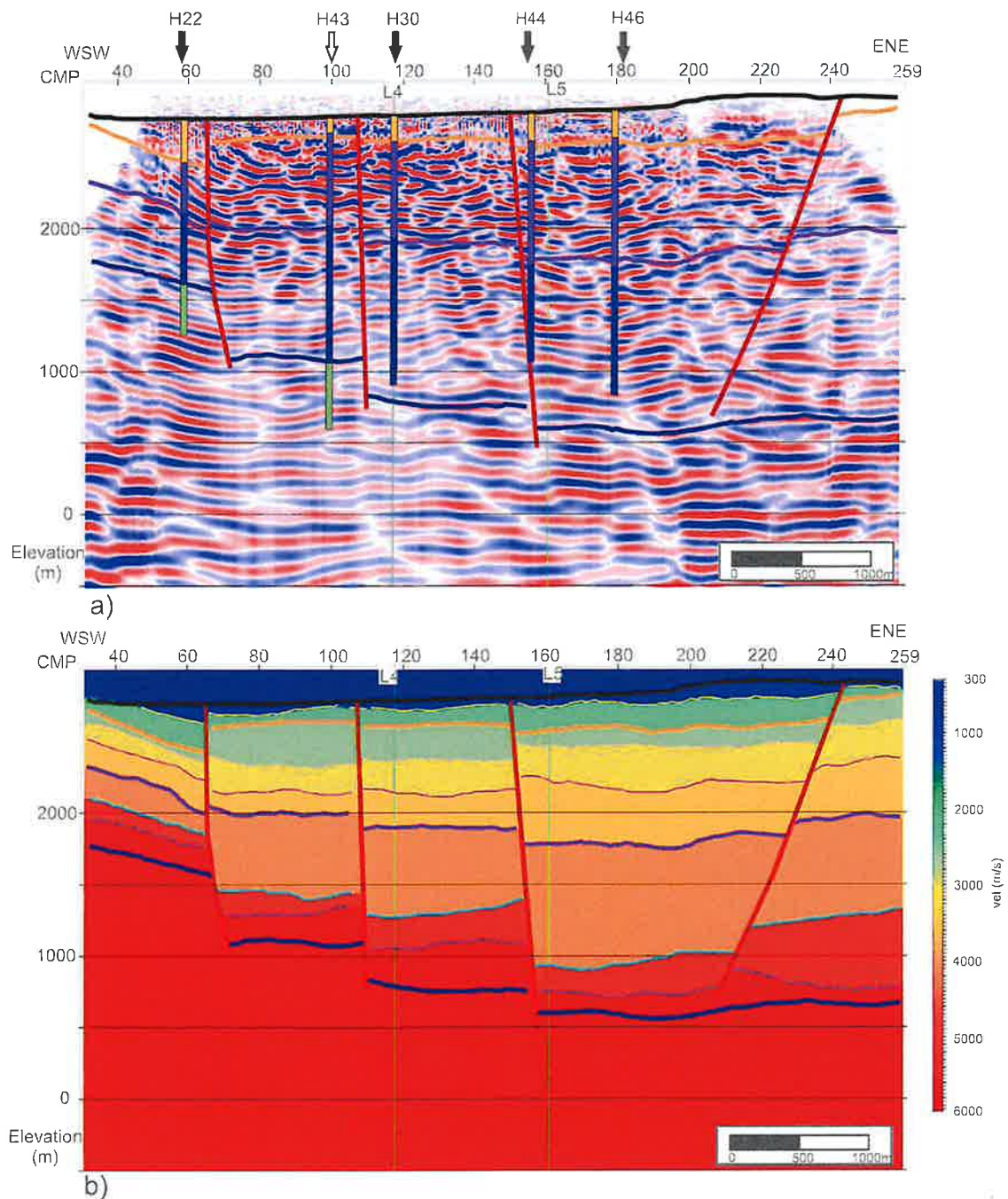
Fig. 13. (a) L2 interpreted depth seismic section with stratigraphic profiles of the used wells. The black arrows indicate wells on the line, the blank arrows indicate wells in the proximity of the line. For the color legend of the horizons and the well stratigraphy see the column "Group" in Fig. 11. (b) 2D depth interval velocity field for line L2. The color legend of the horizons lines is shown in the column "Seismic unit" in Fig. 11. Both in (a) and (b), the green vertical lines indicate the crossing positions with the other lines, the vertical scale is in meters above sea level. (For interpretation of the references to color in this figure legend, the reader is referred to the web version of this article.)
