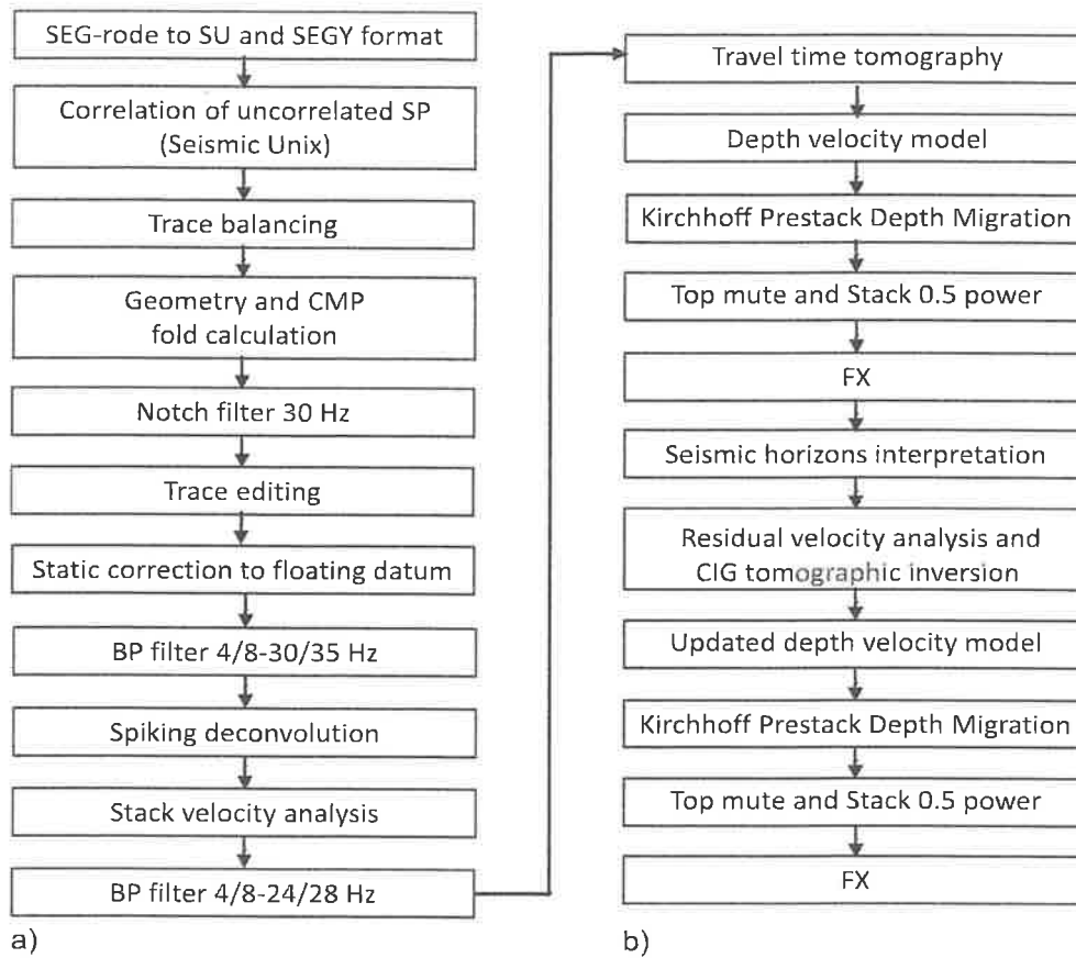
Fig. 5. (a) Time- and (b) depth- processing flows.
