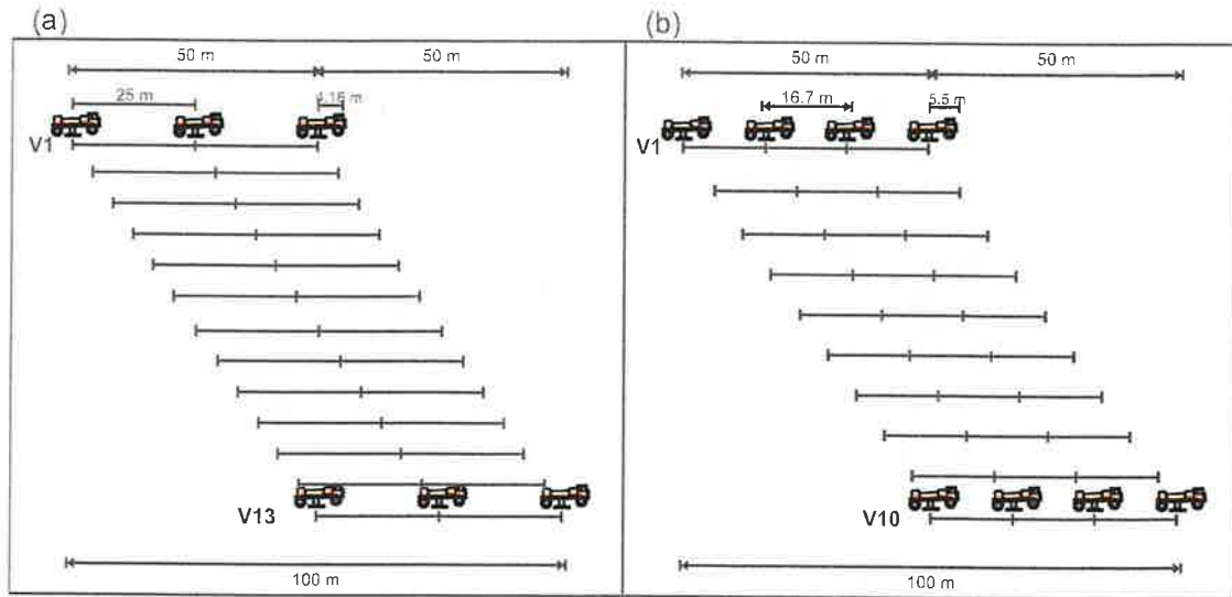
Fig. 3. The two different patterns of vibrations (a) and (b), described in Table 1 (modified after seismic acquisition report; COMESA, 1998).
