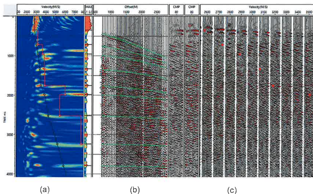
Fig. B.2. Stacking velocity analysis, with (a) semblance, the black line indicates the picked velocity, the red line is the corresponding interval velocity, (b) CMP versus offset gather, the green lines highlight the reflections corresponding to the picked velocity, (c) common velocity stacks, the red dots are the projections on the picked velocities on the stacks. (For interpretation of the references to color in this figure legend, the reader is referred to the web version of this article.)
