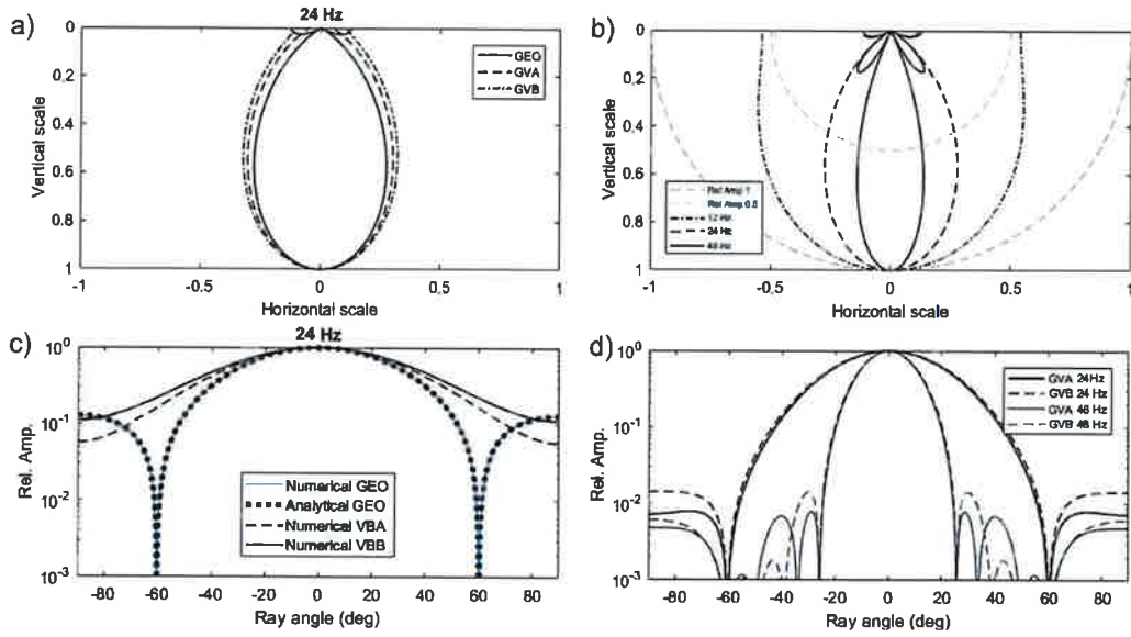
Fig. A.2. Diagrams and responses of the geophone and vibrator arrays. (a) Plot of polar radiation diagrams calculated for geophone, vibrator configuration A (VIB A), vibrator configuration B (VIB B) at the harmonic frequency 24 Hz. (b) Polar plots of the geophone array diagrams calculated at the harmonic frequencies 12, 24, 48 Hz. (c) Array response vs ray angle \alpha (emission or incidence), showing the geophone numerical response, the geophone analytical response together with the VIB A, VIB B responses calculated at 24 Hz. (d) Composition of geophone and vibrator (GVA and GVB in vibrator configuration A and B, respectively) array's responses vs ray angle \alpha , for plane harmonic waves at frequencies 24 and 48 Hz.
