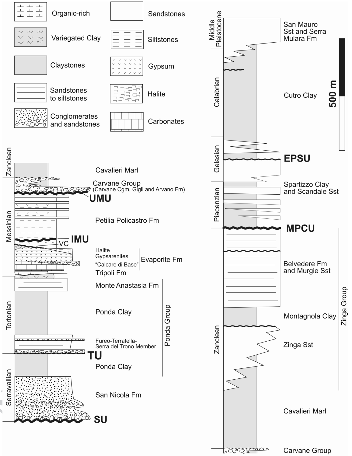
Figure 2. Simplified stratigraphy of the Crotonese Basin and its onshore sector (modified from Zecchin et al. 19 ). Formations and unconformities are shown in the figure. SU Basal Unconformity, EPSU Early Pleistocene Unconformity, IMU Intra-Messinian Unconformity, MPCU Mid-Pliocene Unconformity, TU Tortonian Unconformity, UMU Upper Messinian Unconformity.
