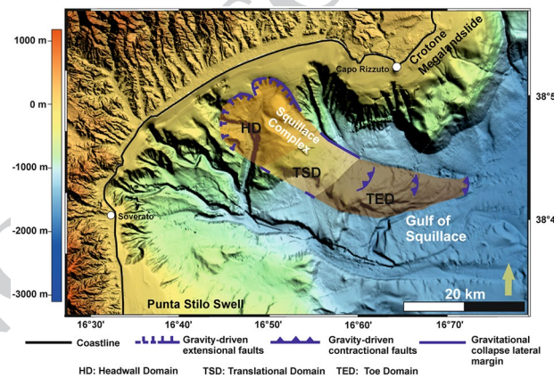
Figure 9. Bathymetric data highlighting the scale of the Squillace Complex within the Gulf of Squillace. The Headwall (HD), translational (TSD) and toe (TED) domains of the complex are mapped in detail. See captions Fig. 1B in order to see where the DTM was obtained from.
